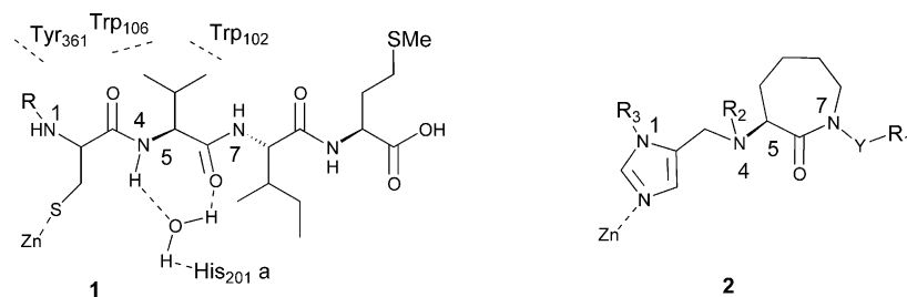
Figure 1. Interactions of compound 1 with FTase and structures of compounds 1 and 2 .
