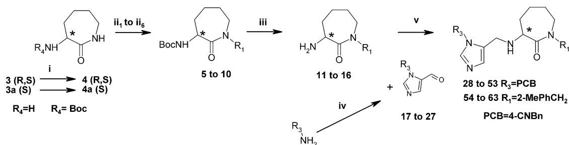
Scheme 1. Synthesis of compounds 28–63 . (i): (Boc) 2 O, NaOH, H 2 O/tBuOH, rt, 12 h, ( 4 , 88%); (ii 1 ) (a) BiPh 3 , pyridine, Cu(OAc) 2 , CH 2 Cl 2 , rt, 24 h ( 5 , 77%); (ii 2 ) (a) NaH THF/DMF, 0 °C, 30 min; (b) PhCH 2 Br, N(Bu) 4 , I, rt, 24 h ( 6 , 97%). (ii 3 ) (a) NaH, DMF, 0 °C, 30 min; (b) Ph(CH 2 ) 2 OTs, 0 °C, 12 h ( 7 , 75%); (ii 4 ) (a) NaH DMF, 0 °C, 30 min, rt, 2 h; (b) Ph(CH 2 ) 3 OTs, rt, 12 h ( 8 , 86%); (ii 5 ) (a) LiHMDS, 0 °C, 15 min; (b) PhSO 2 Cl, 0 °C, rt, 2 h ( 9 , 77%); (ii 6 ) (a) PhSCH 2 Cl, KOH, N(Bu) 4 I, THF, rt, 12 h; (b) dimethyldioxirane, acetone, 0 °C, rt, 2 h, ( 10 , 40%); (iii) TFA, CH 2 Cl 2 , 0 °C, rt, 2 h or 4 N HCl/dioxane, rt ( 11–16 ); (iv) (a) dihydroxyacetone dimer, KSCN, MeCN/EtCO 2 H, 60 °C, 2 h; (b) H 2 O 2 , H 2 O, 40 °C, 2 h; (c) DMSO, SO 3 /pyridine, NEt 3 , rt, 2 h ( 17–27 ; Tables 4 and 6); (v) (a) 17–27 , NaBH(OAc) 3 , CH 2 Cl 2 , 0 °C, rt, 12 h; (b) HCl, ether, or fumaric acid, EtOH ( 28–33 ; Table 1; 34–53 ; Tables 2 and 7; 54 to 63 ; Tables 4 and 8).
